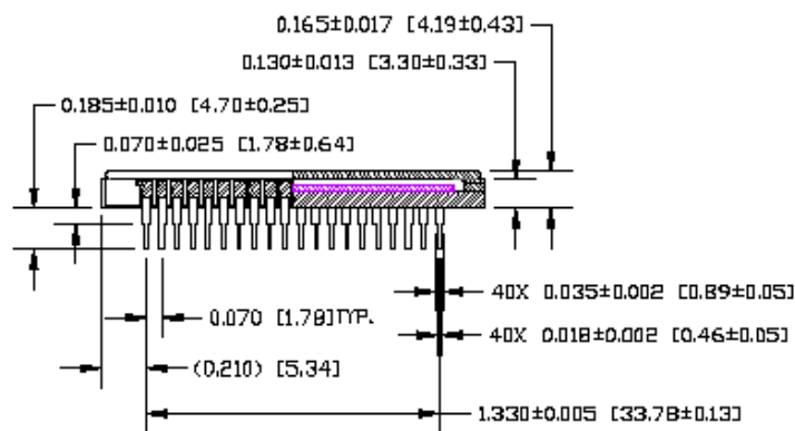
Figure 33: Package Drawing
