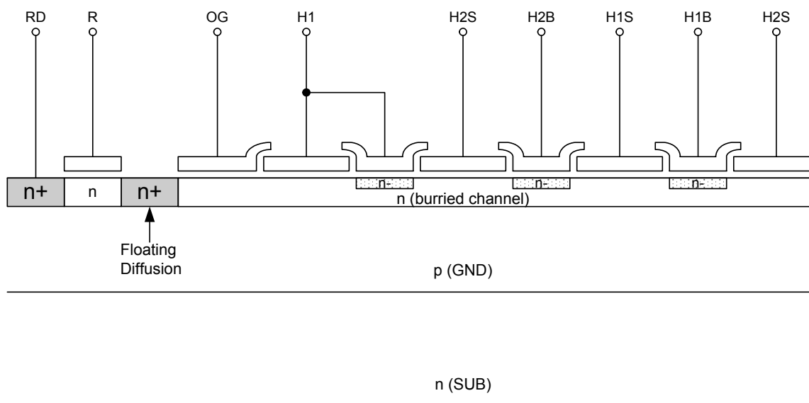
Figure 4: Horizontal Register to Floating Diffusion Architecture
