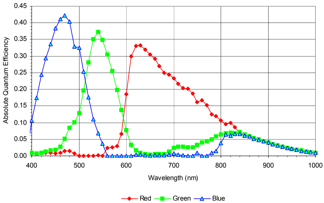
Figure 10: Color with Microlens Quantum Efficiency Using AR Glass
