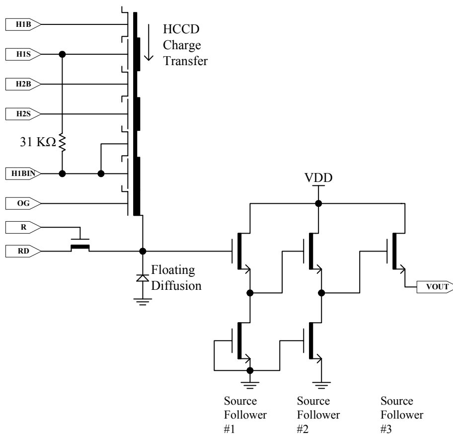
Figure 6: Output Architecture
